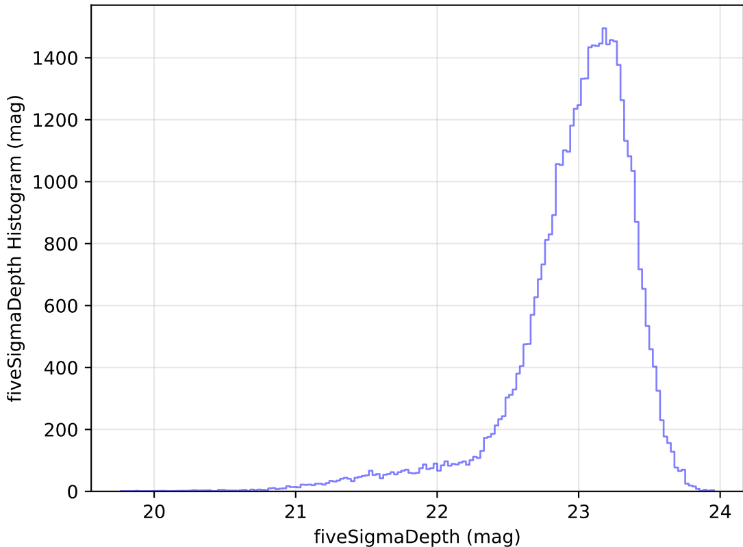
too_elab_r8_d3_griz_v3.4_10yrs Yr 1 z band: fiveSigmaDepth Histogram
