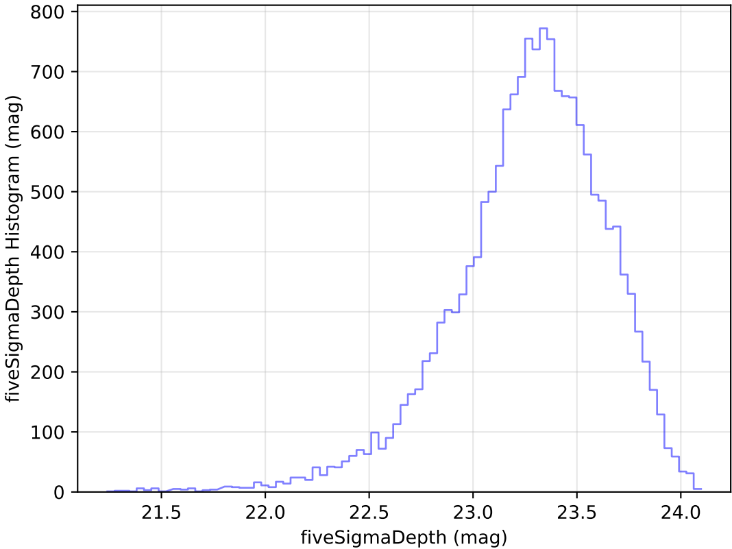
too_elab_r8_d3_griz_v3.4_10yrs Yr 1 u band: fiveSigmaDepth Histogram
