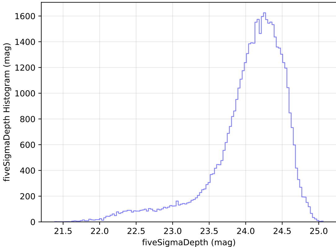
too_elab_r8_d3_griz_v3.4_10yrs Yr 1 r band: fiveSigmaDepth Histogram
