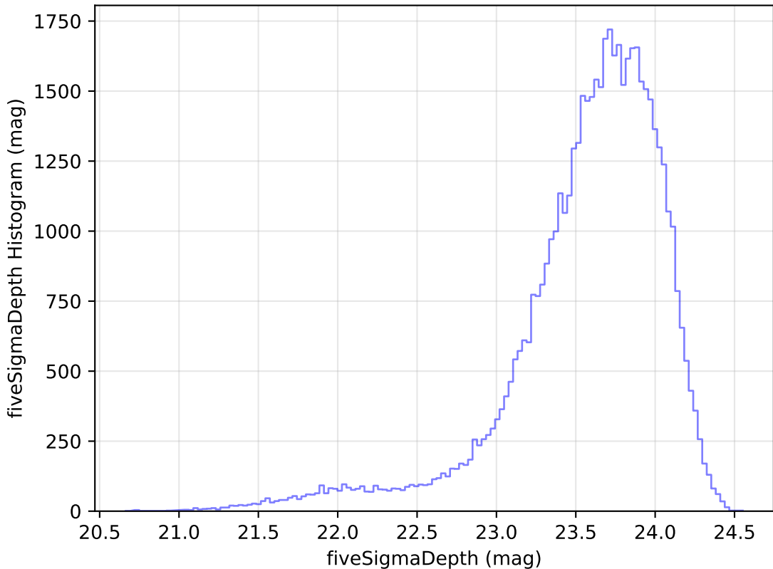
too_elab_r8_d3_griz_v3.4_10yrs Yr 1 i band: fiveSigmaDepth Histogram
