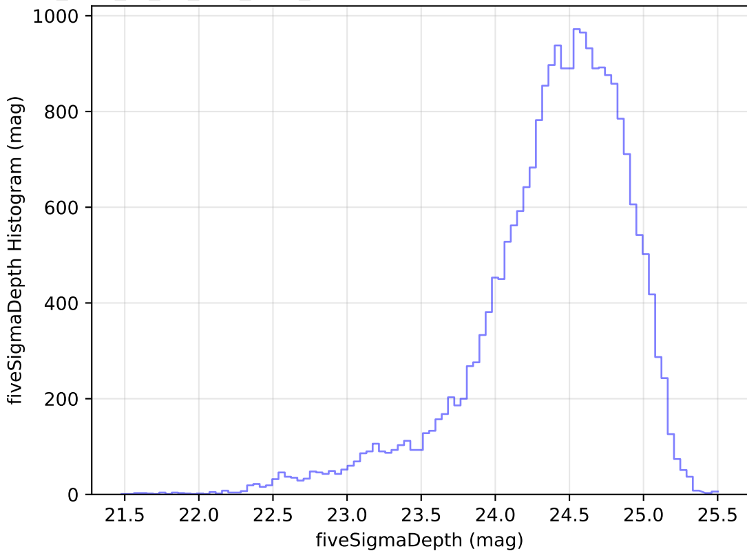
too_elab_r8_d3_griz_v3.4_10yrs Yr 1 g band: fiveSigmaDepth Histogram
