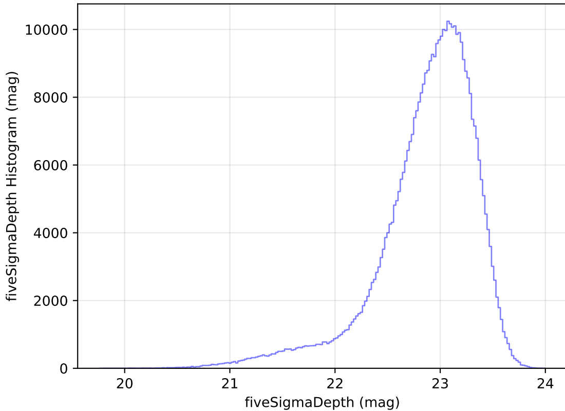
too_elab_r8_d3_griz_v3.4_10yrs WFD z band: fiveSigmaDepth Histogram
