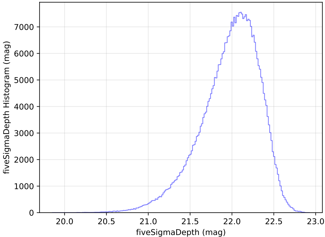
too_elab_r8_d3_griz_v3.4_10yrs WFD y band: fiveSigmaDepth Histogram
