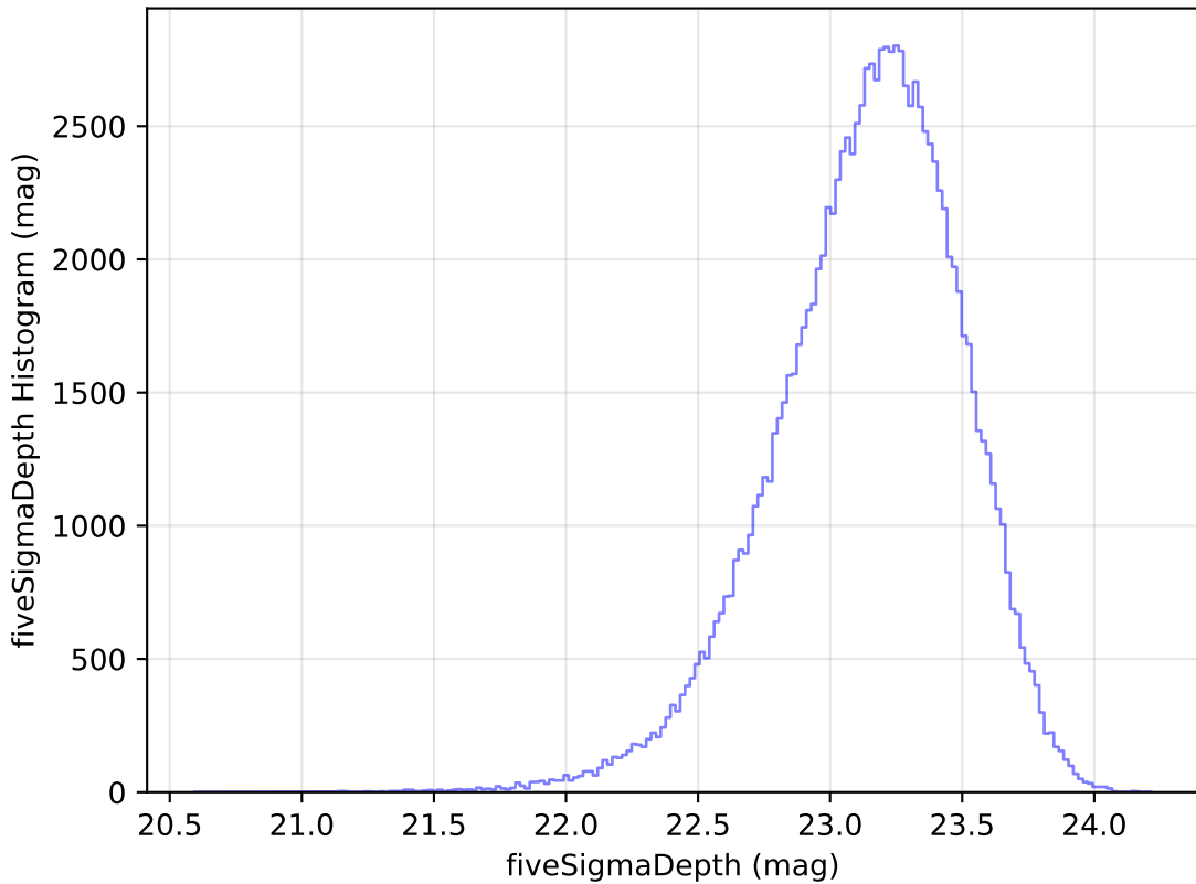
too_elab_r8_d3_griz_v3.4_10yrs WFD u band: fiveSigmaDepth Histogram
