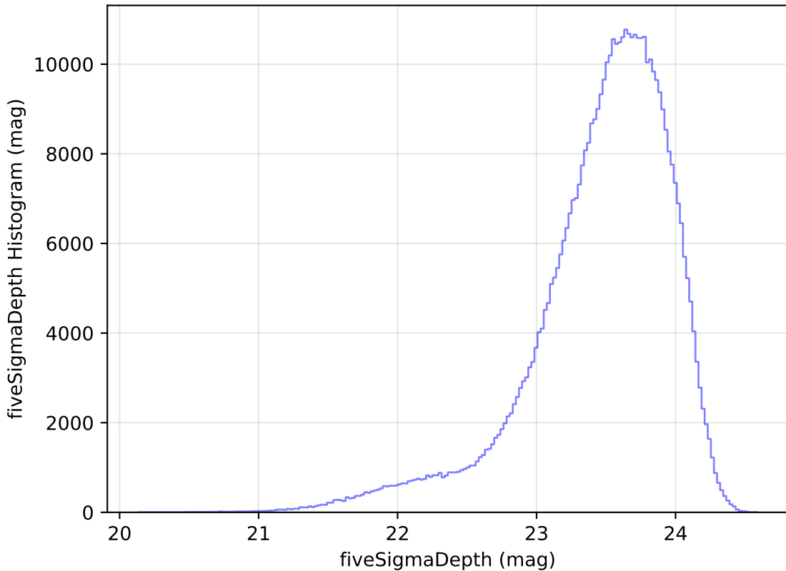
too_elab_r8_d3_griz_v3.4_10yrs WFD i band: fiveSigmaDepth Histogram
