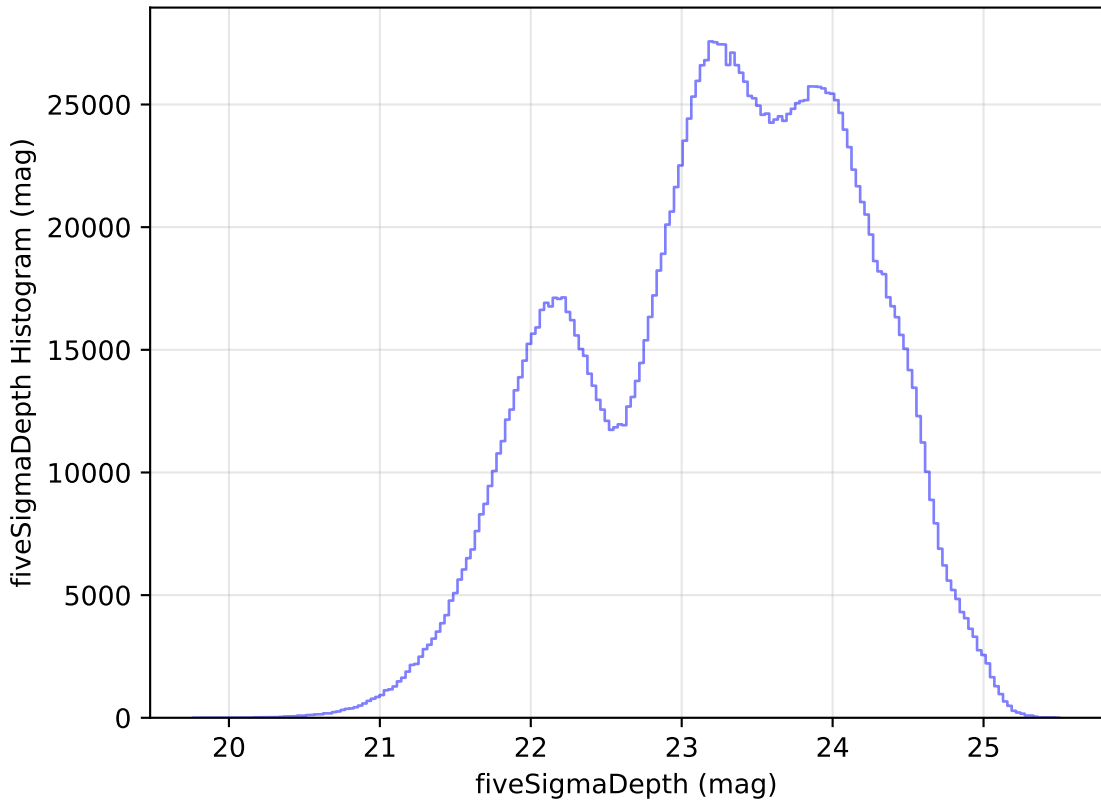
too_elab_r8_d3_griz_v3.4_10yrs WFD all bands: fiveSigmaDepth Histogram
