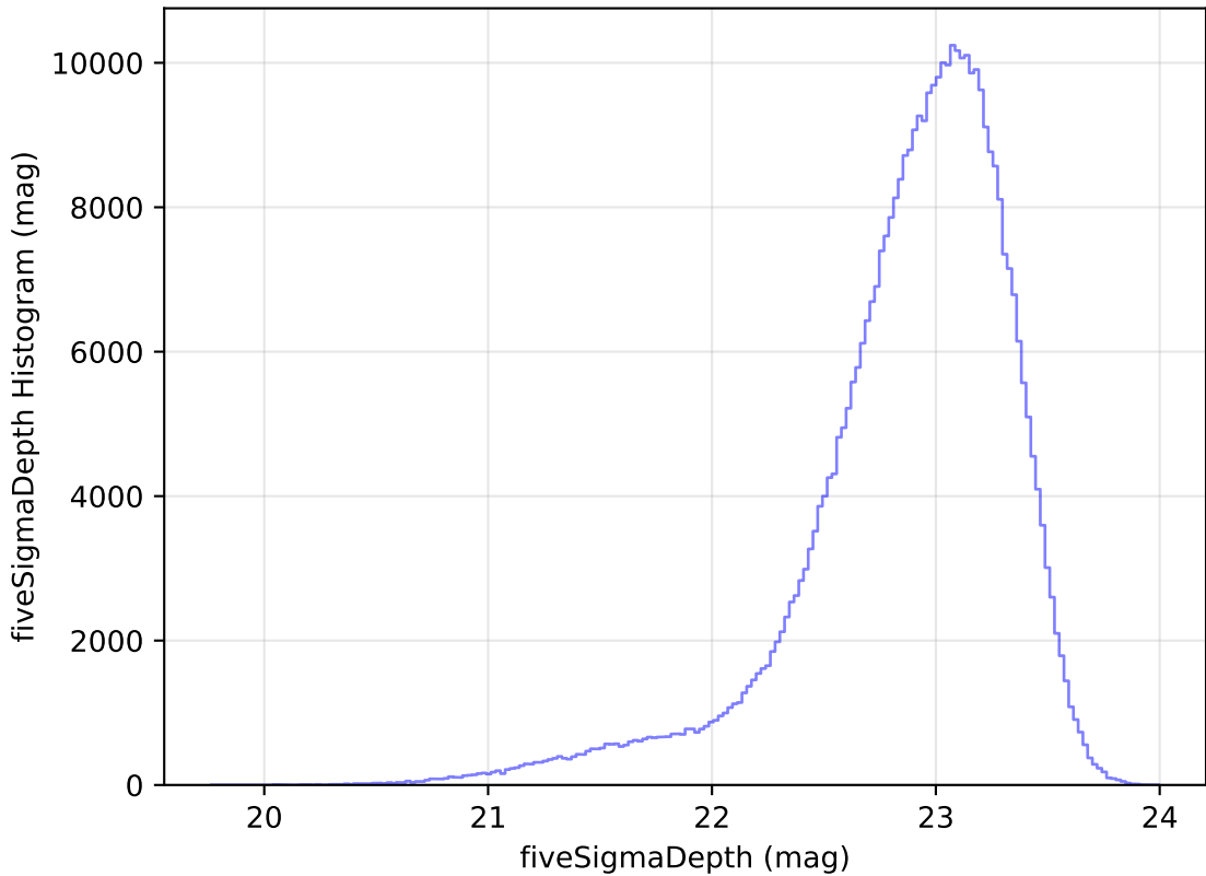
too_elab_r8_d3_griz_v3.4_10yrs All sky z band: fiveSigmaDepth Histogram
