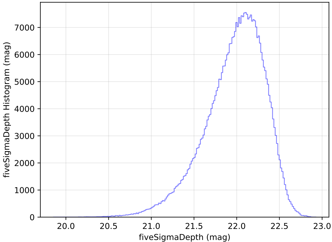
too_elab_r8_d3_griz_v3.4_10yrs All sky y band: fiveSigmaDepth Histogram
