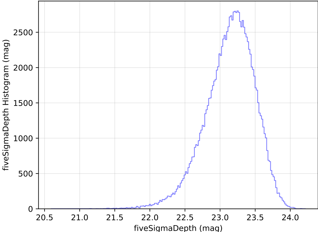
too_elab_r8_d3_griz_v3.4_10yrs All sky u band: fiveSigmaDepth Histogram
