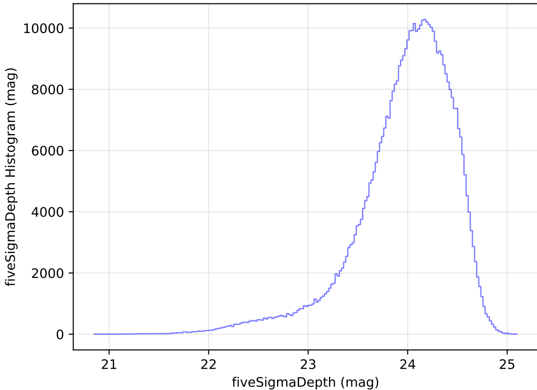
too_elab_r8_d3_griz_v3.4_10yrs All sky r band: fiveSigmaDepth Histogram
