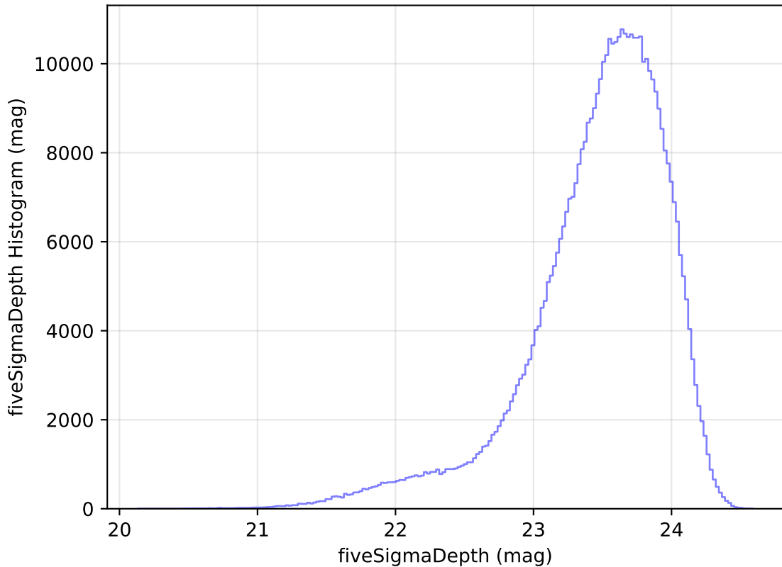
too_elab_r8_d3_griz_v3.4_10yrs All sky i band: fiveSigmaDepth Histogram
