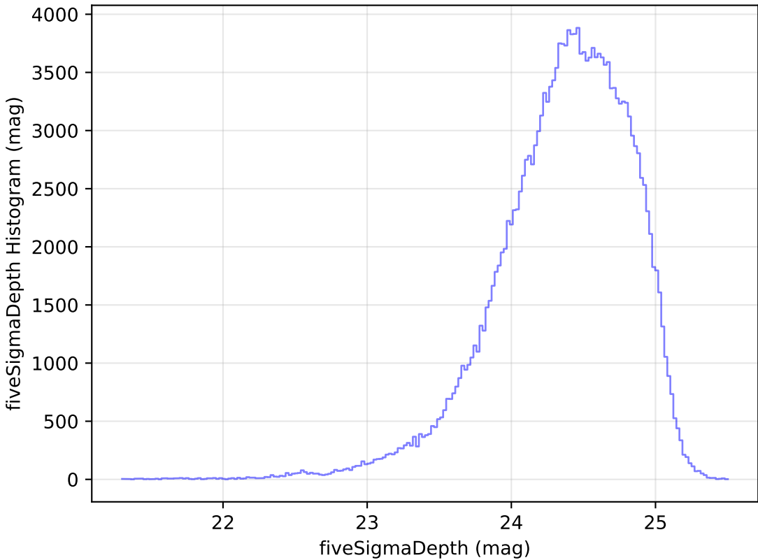
too_elab_r8_d3_griz_v3.4_10yrs All sky g band: fiveSigmaDepth Histogram
