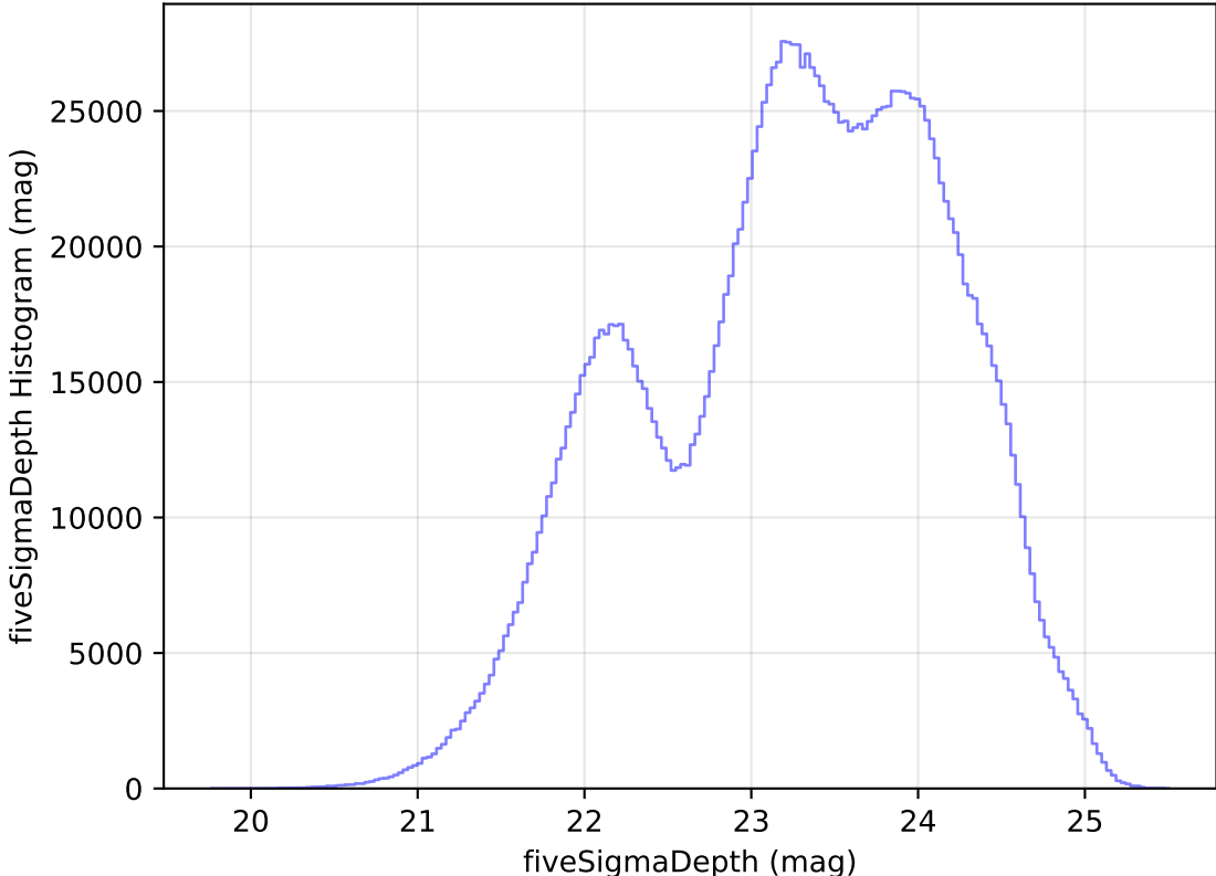
too_elab_r8_d3_griz_v3.4_10yrs All sky all bands: fiveSigmaDepth Histogram
