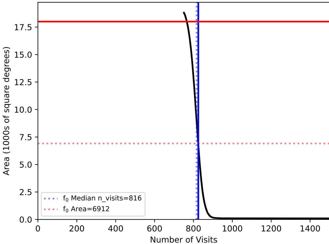
too_elab_r8_d3_griz_v3.4_10yrs WFD: fO
