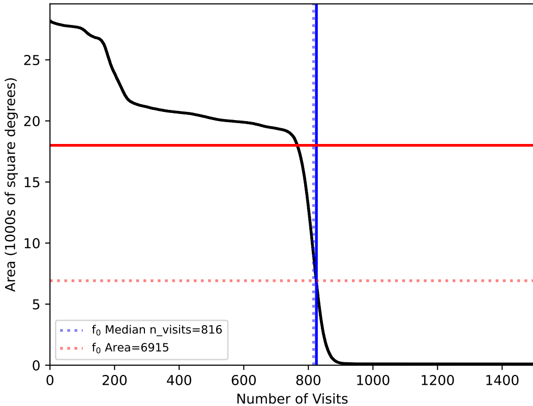
too_elab_r8_d3_griz_v3.4_10yrs All sky: f0
