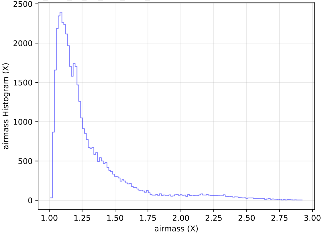
too_elab_r8_d3_griz_v3.4_10yrs Yr 1 z band: airmass Histogram
