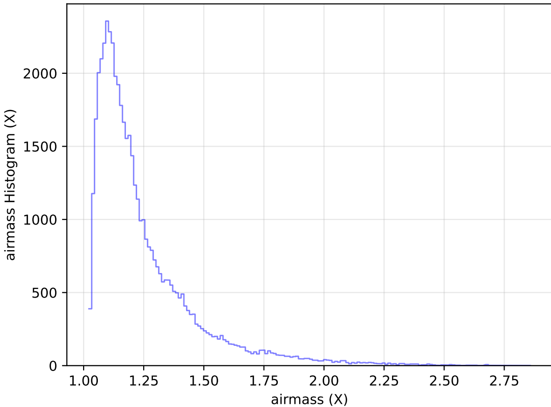
too_elab_r8_d3_griz_v3.4_10yrs Yr 1 y band: airmass Histogram
