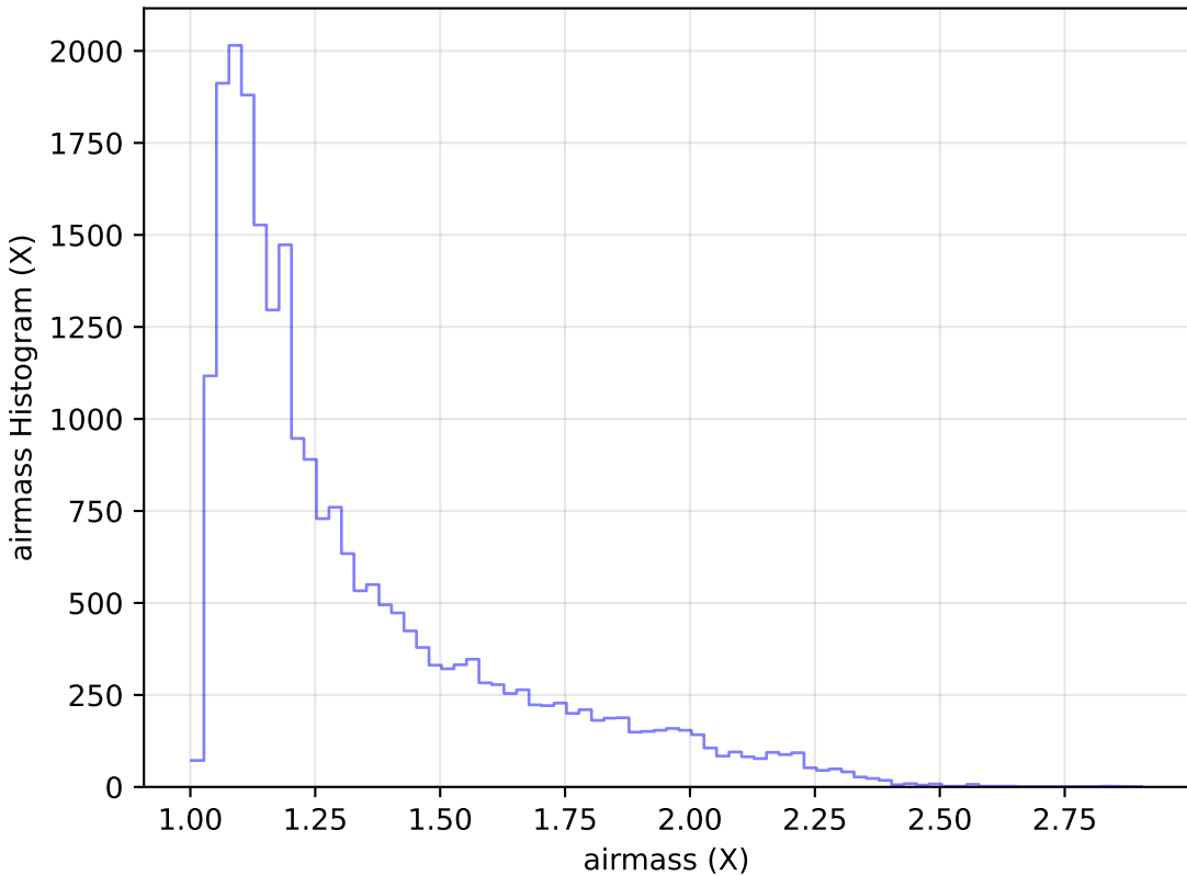
too_elab_r8_d3_griz_v3.4_10yrs Yr 1 g band: airmass Histogram
