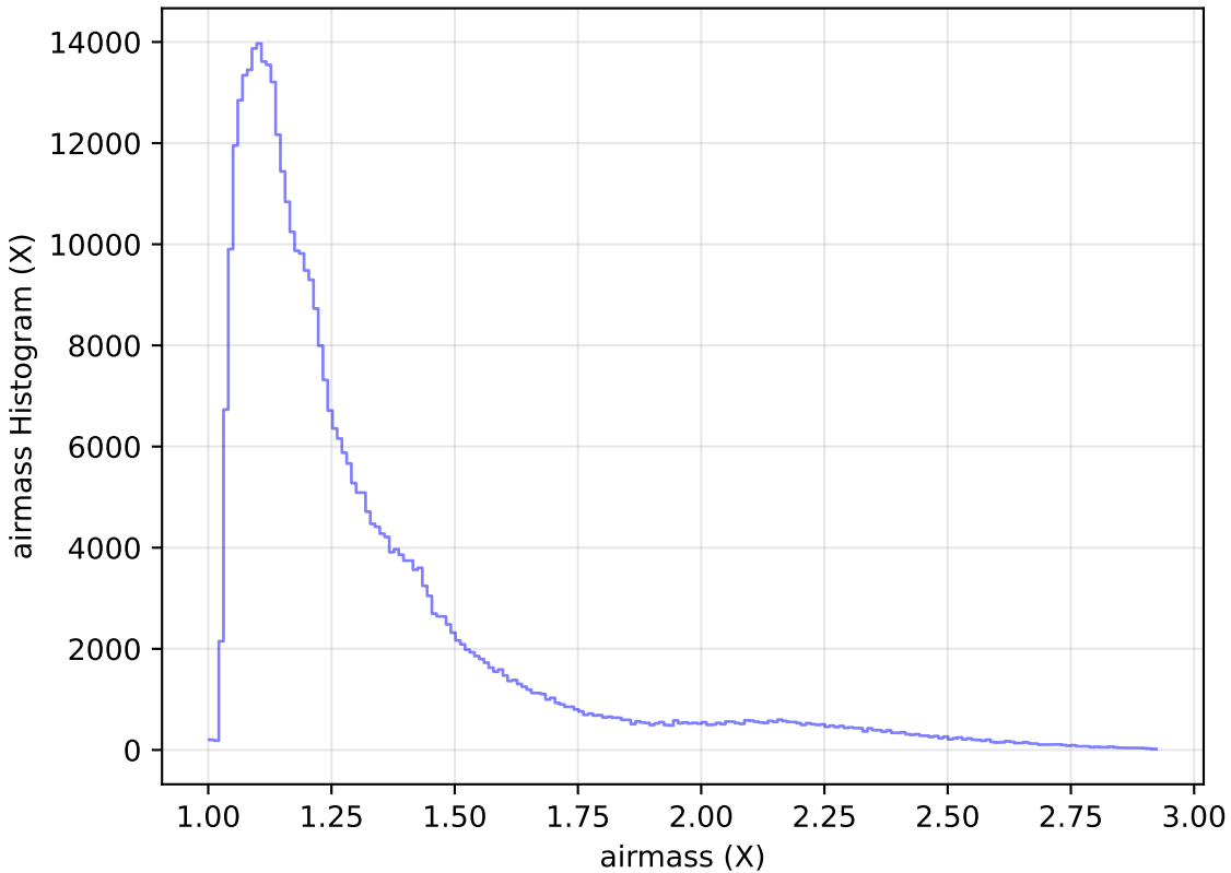
too_elab_r8_d3_griz_v3.4_10yrs WFD z band: airmass Histogram
