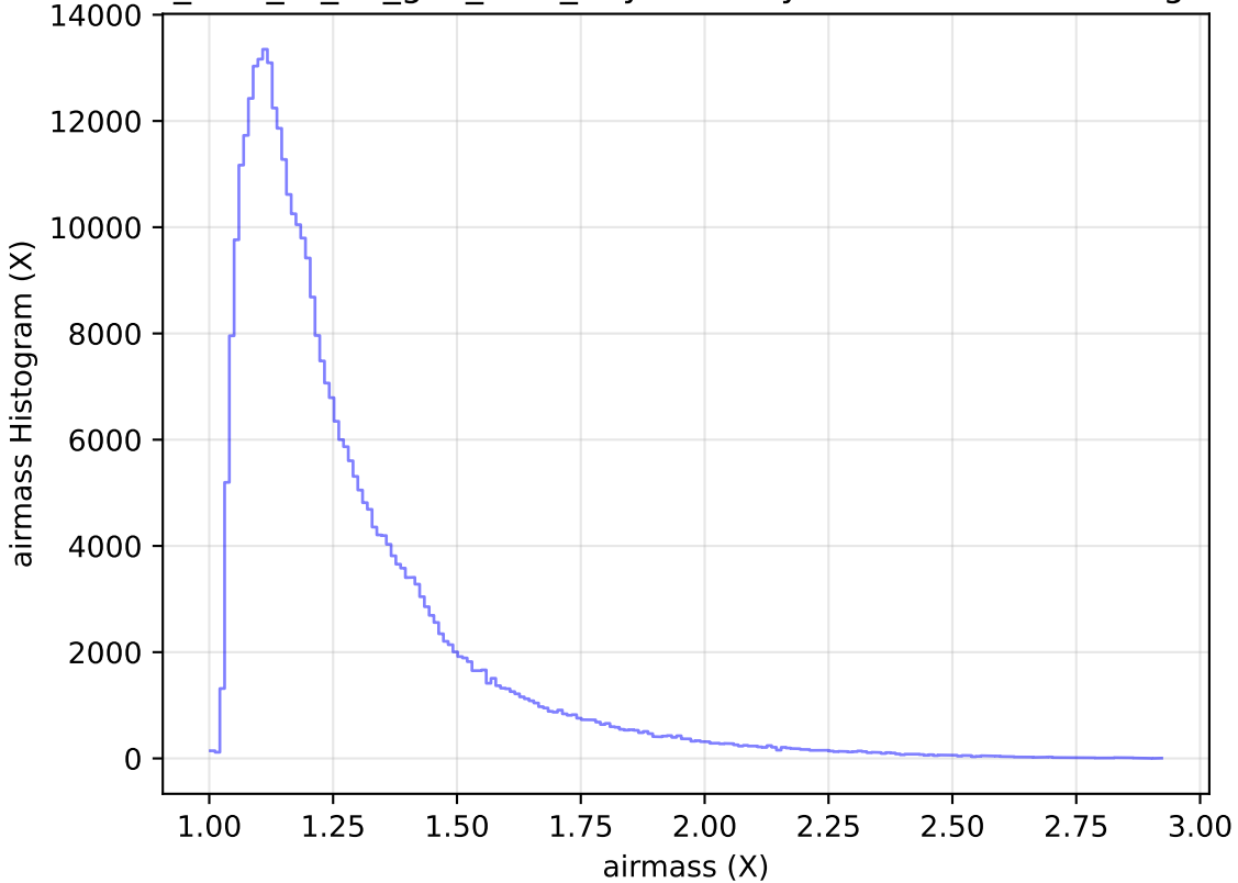
too_elab_r8_d3_griz_v3.4_10yrs WFD y band: airmass Histogram
