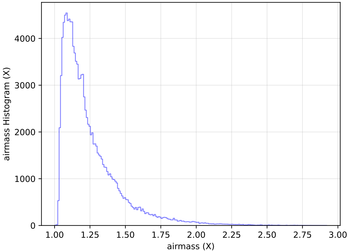
too_elab_r8_d3_griz_v3.4_10yrs WFD u band: airmass Histogram
