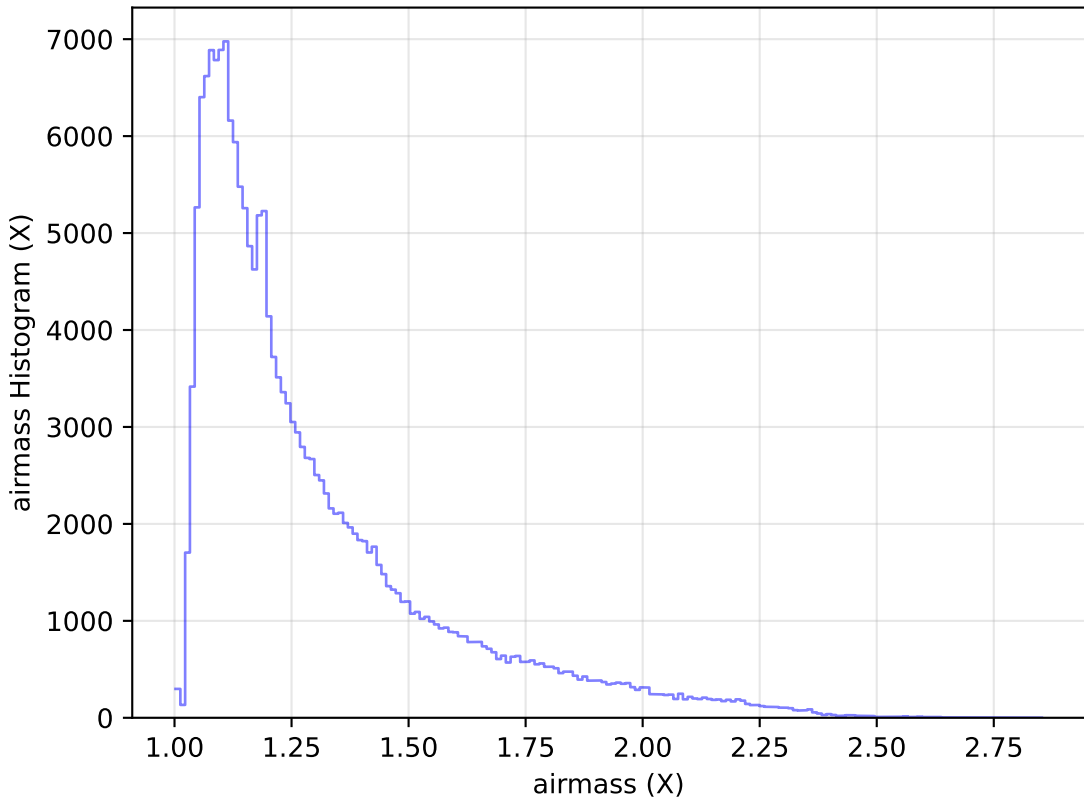
too_elab_r8_d3_griz_v3.4_10yrs WFD g band: airmass Histogram
