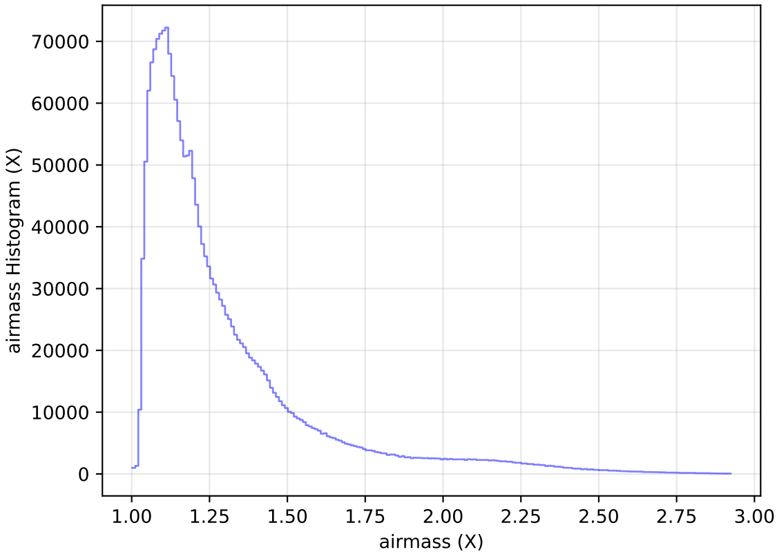
too_elab_r8_d3_griz_v3.4_10yrs WFD all bands: airmass Histogram
