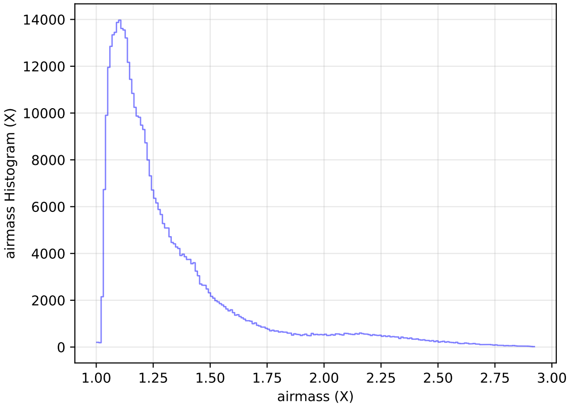
too_elab_r8_d3_griz_v3.4_10yrs All sky z band: airmass Histogram
