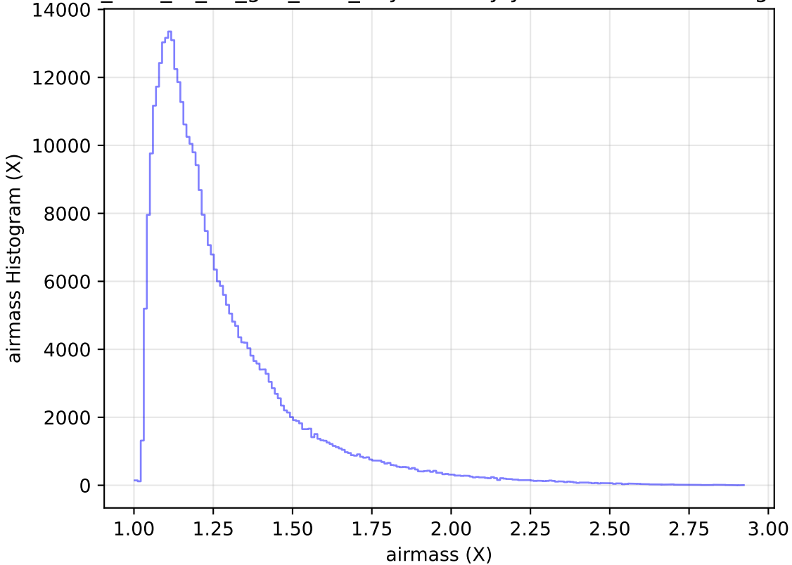
too_elab_r8_d3_griz_v3.4_10yrs All sky y band: airmass Histogram
