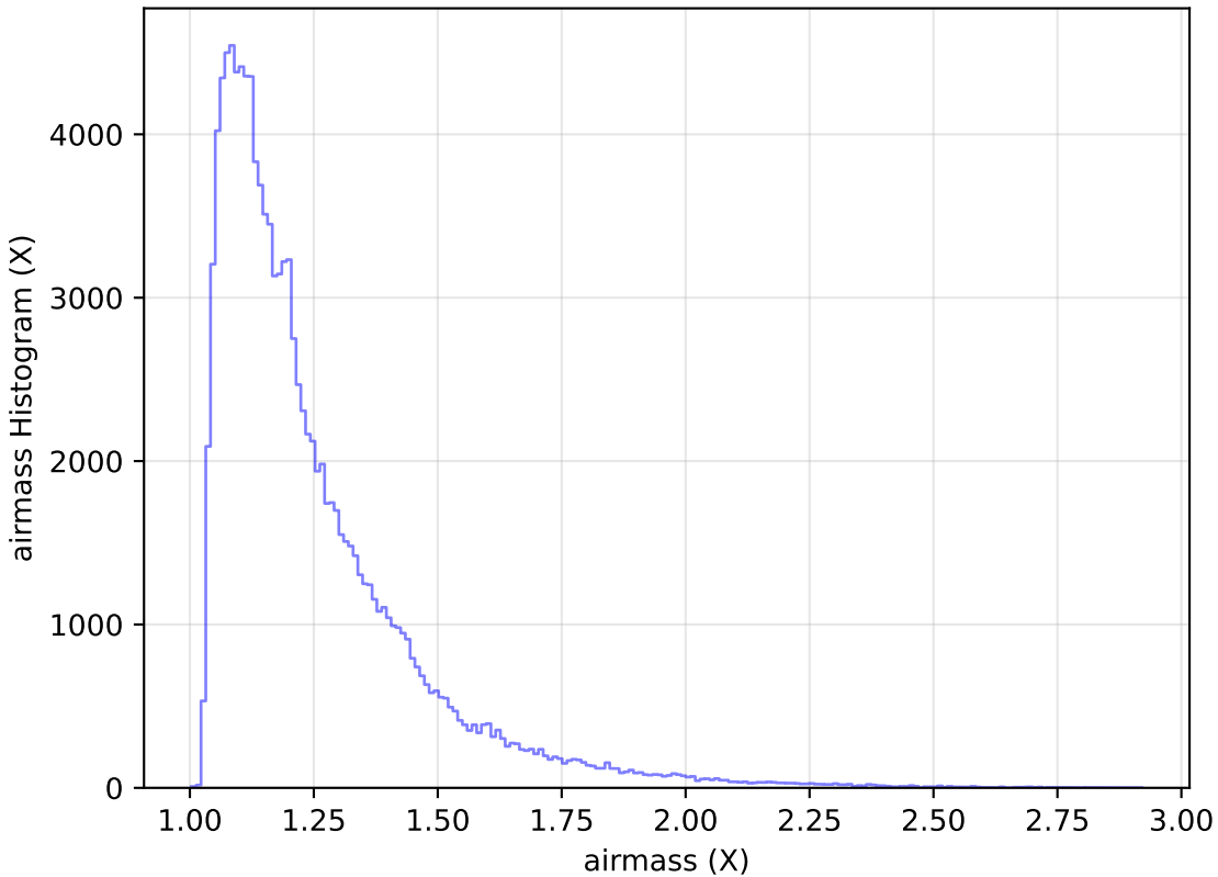
too_elab_r8_d3_griz_v3.4_10yrs All sky u band: airmass Histogram
