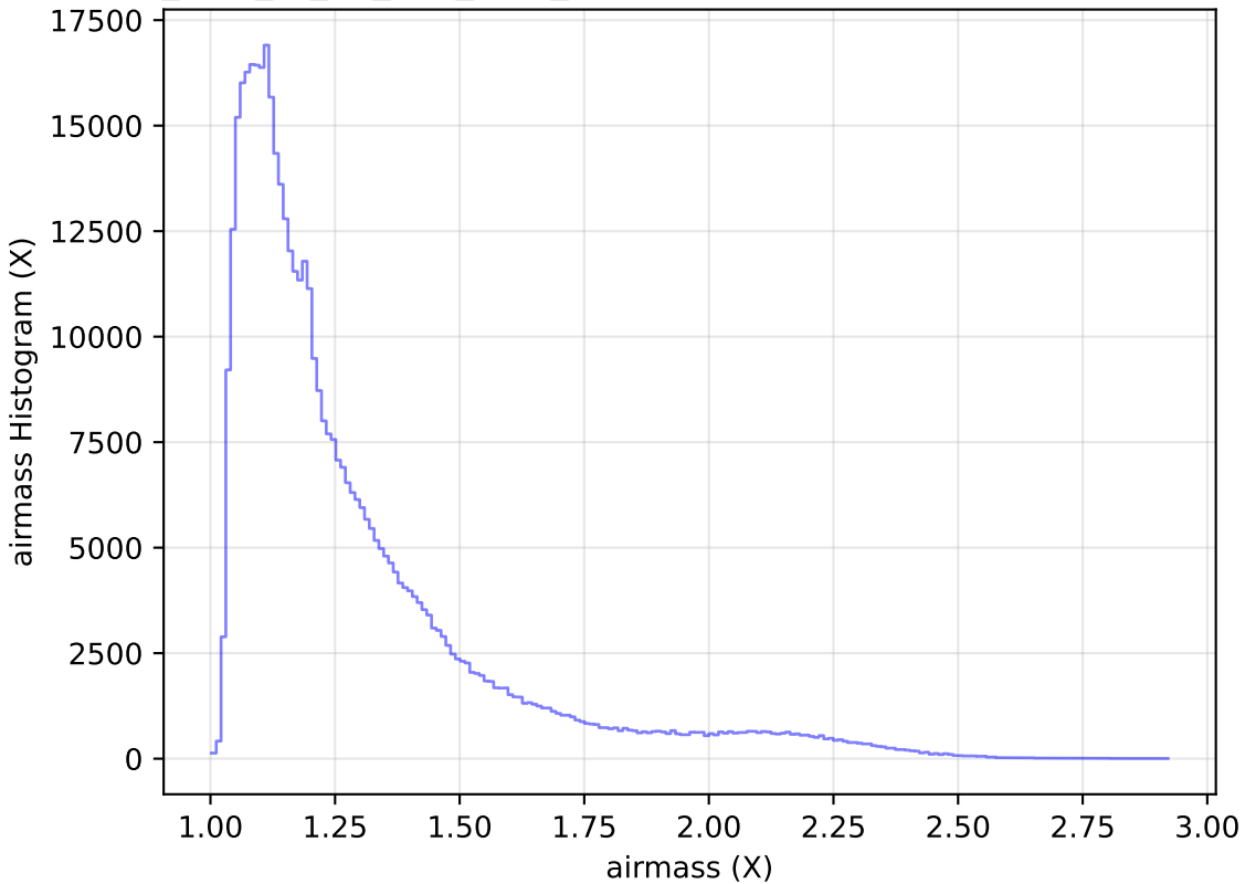
too_elab_r8_d3_griz_v3.4_10yrs All sky r band: airmass Histogram
