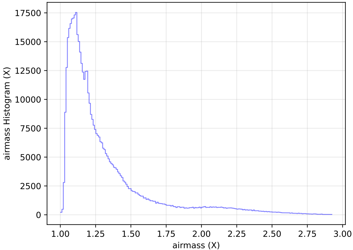
too_elab_r8_d3_griz_v3.4_10yrs All sky i band: airmass Histogram
