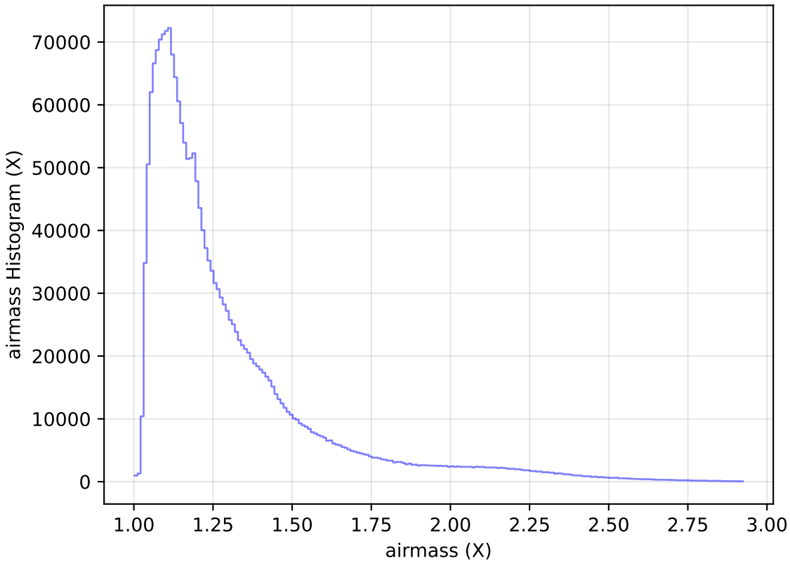
too_elab_r8_d3_griz_v3.4_10yrs All sky all bands: airmass Histogram
