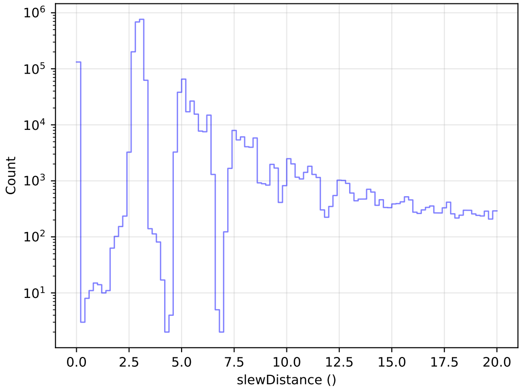
too_elab_r8_d3_griz_v3.4_10yrs All visits: Zoom Slew Distance Histogram
