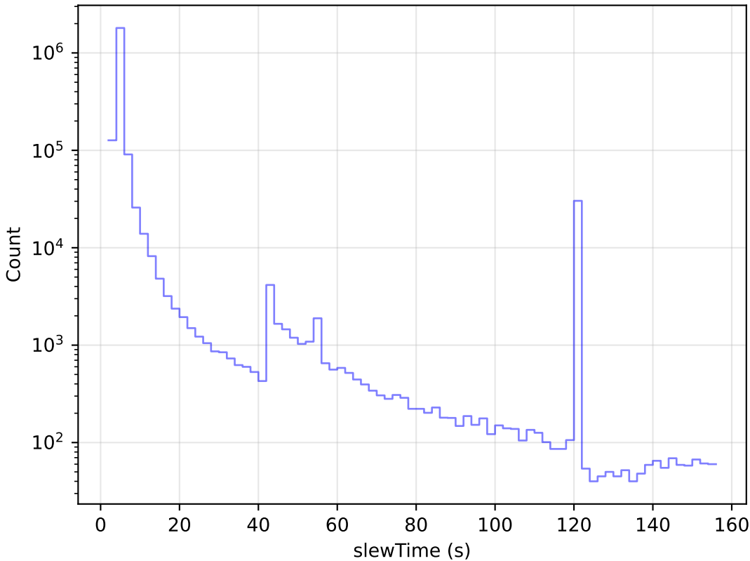
too_elab_r8_d3_griz_v3.4_10yrs All visits: Slew Time Histogram
