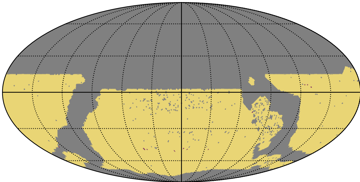
too_elab_r8_d3_griz_v3.4_10yrs WFD: RapidRevisits
