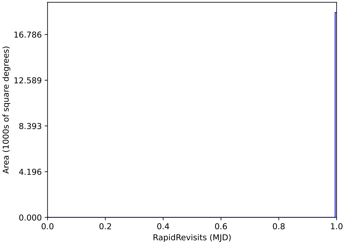
too_elab_r8_d3_griz_v3.4_10yrs WFD: RapidRevisits
