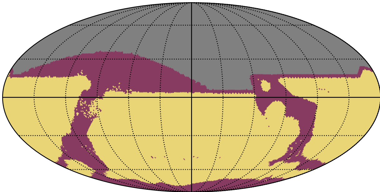
too_elab_r8_d3_griz_v3.4_10yrs All sky: RapidRevisits
