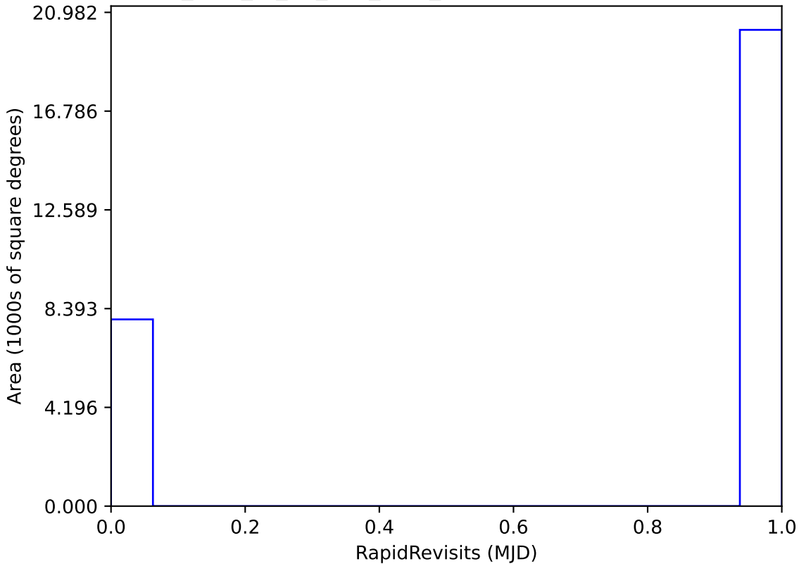
too_elab_r8_d3_griz_v3.4_10yrs All sky: RapidRevisits
