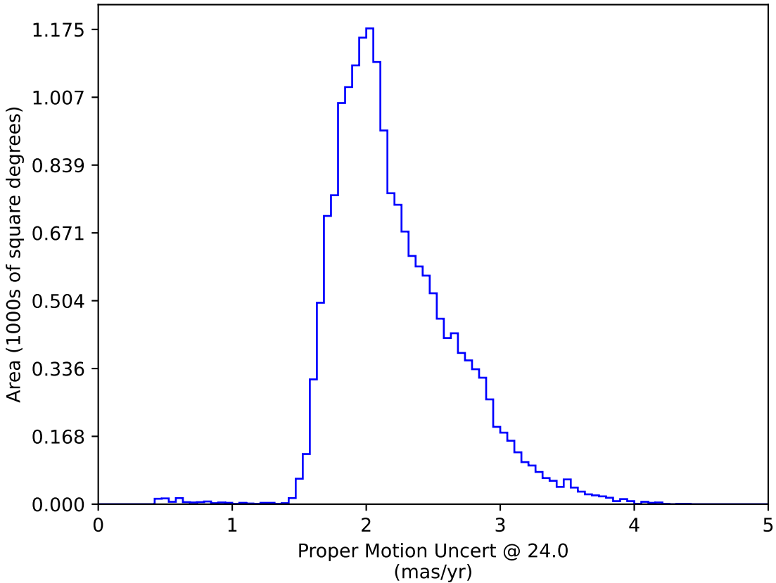
too_elab_r8_d3_griz_v3.4_10yrs WFD: Proper Motion Uncert @ 24.0
