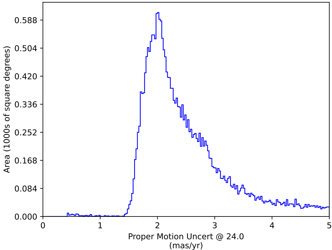
too_elab_r8_d3_griz_v3.4_10yrs All sky: Proper Motion Uncert @ 24.0
