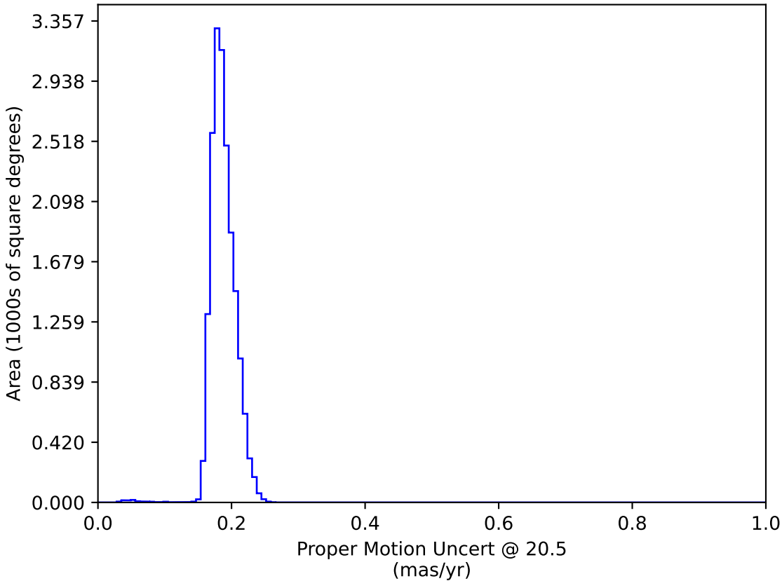
too_elab_r8_d3_griz_v3.4_10yrs WFD: Proper Motion Uncert @ 20.5
