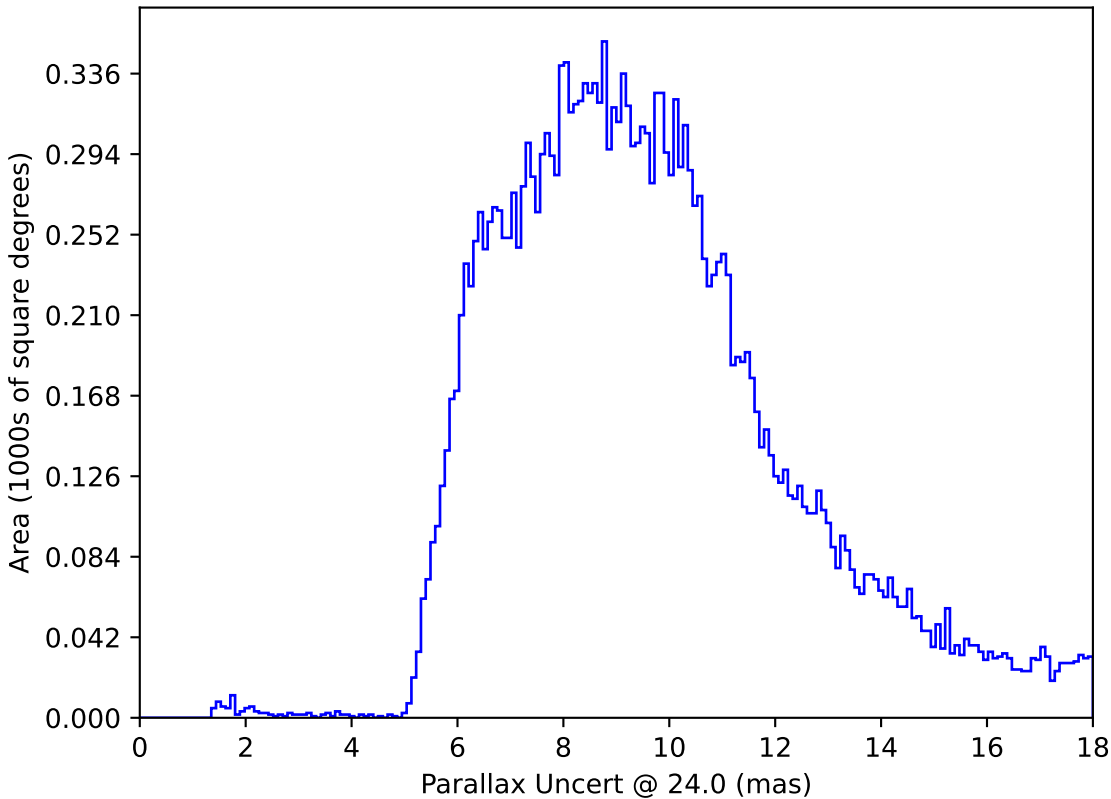
too_elab_r8_d3_griz_v3.4_10yrs All sky: Parallax Uncert @ 24.0
