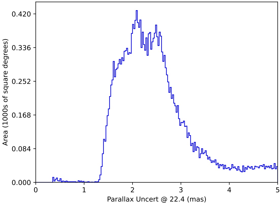
too_elab_r8_d3_griz_v3.4_10yrs All sky: Parallax Uncert @ 22.4
