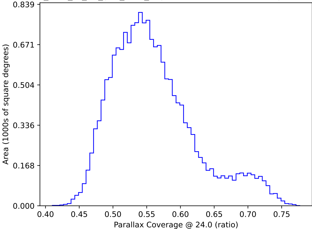
too_elab_r8_d3_griz_v3.4_10yrs WFD: Parallax Coverage @ 24.0
