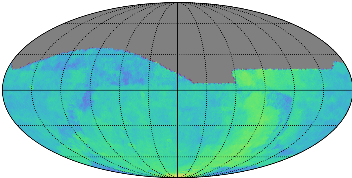
too_elab_r8_d3_griz_v3.4_10yrs All sky: Parallax Coverage @ 24.0
