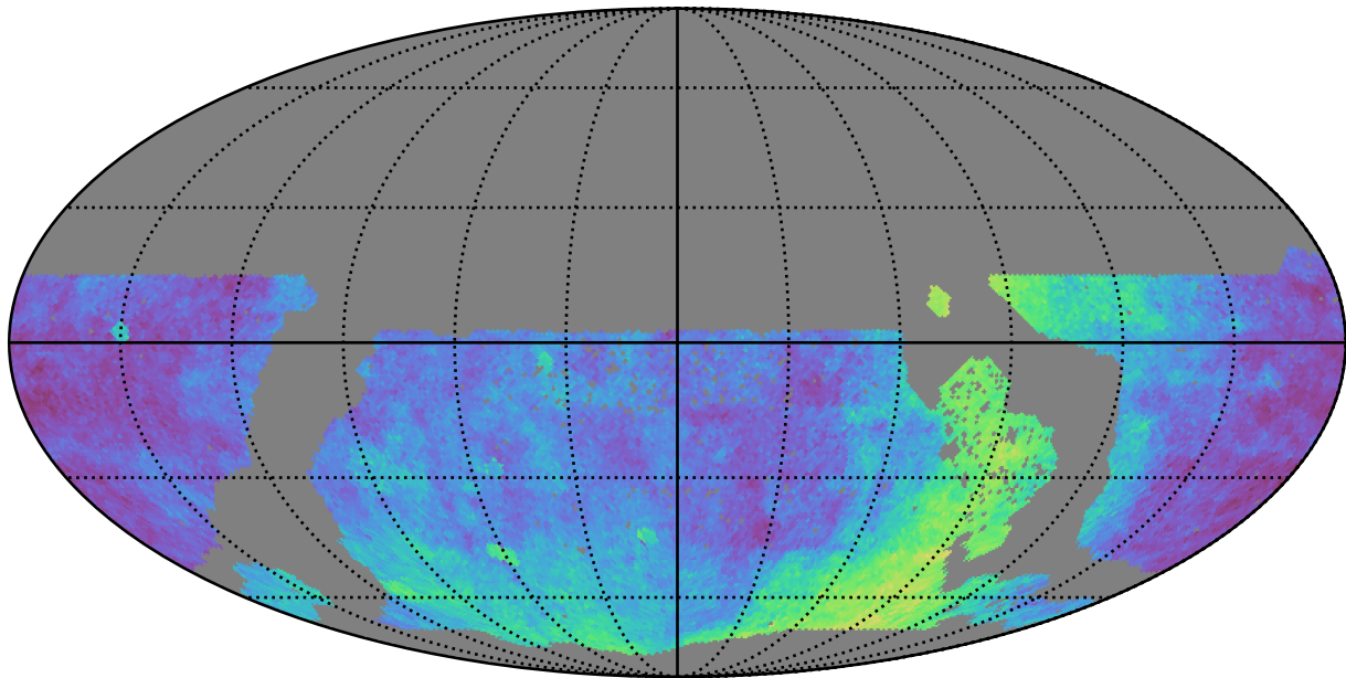
too_elab_r8_d3_griz_v3.4_10yrs WFD: Parallax Coverage @ 22.4
