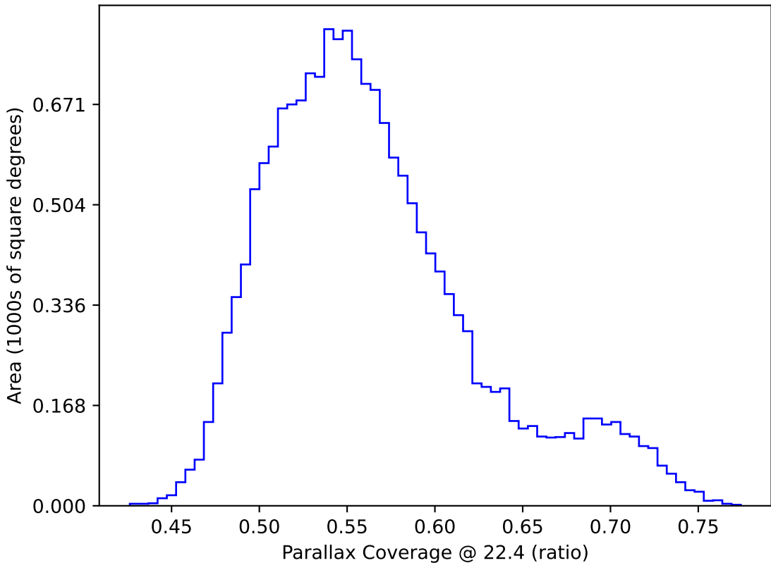
too_elab_r8_d3_griz_v3.4_10yrs WFD: Parallax Coverage @ 22.4
