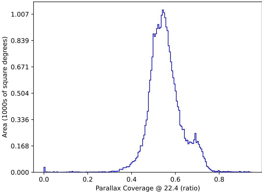
too_elab_r8_d3_griz_v3.4_10yrs All sky: Parallax Coverage @ 22.4
