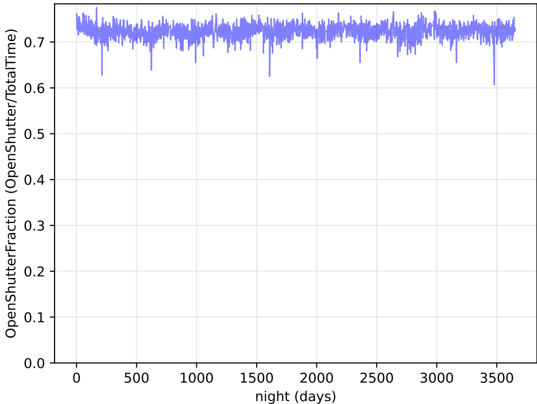
too_elab_r8_d3_griz_v3.4_10yrs Per night: OpenShutterFraction
